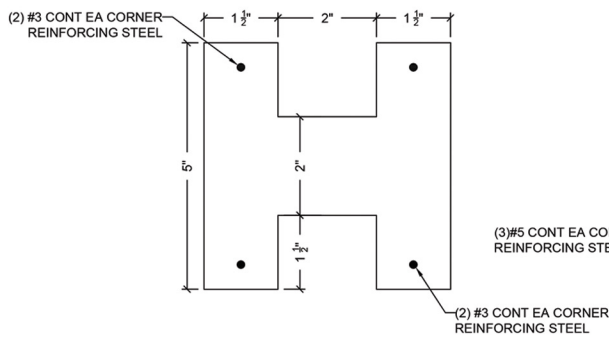
7 COLUMN SECTION 5x5 SCALE: 6"=1'-0"
