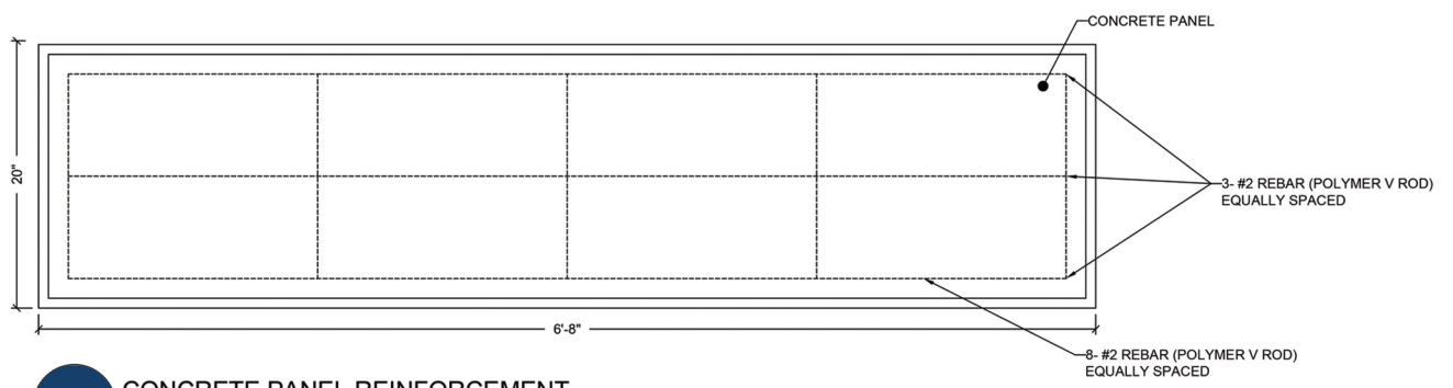
12 CONCRETE PANEL REINFORCEMENT SCALE: 1 \frac{1}{2}''=1'-0''
