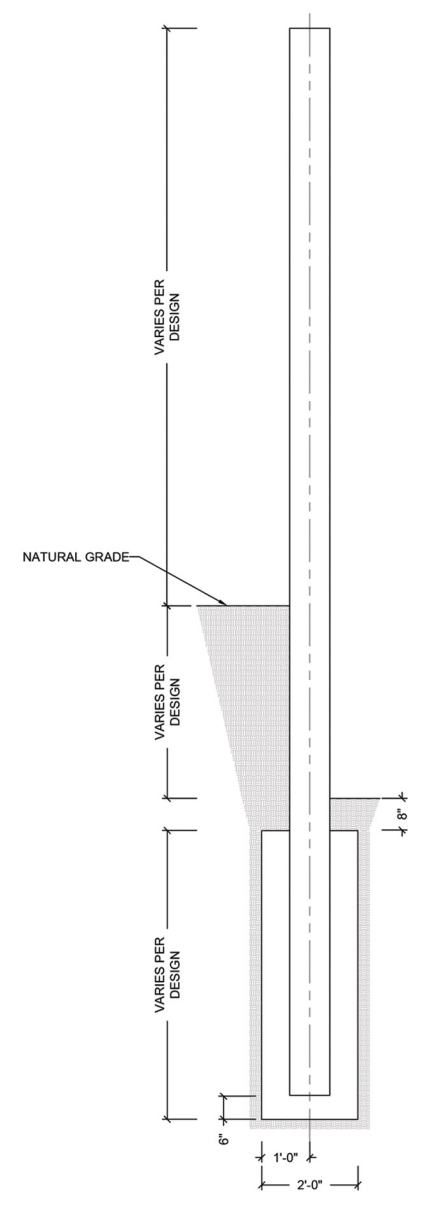
3 FENCE SECTION SCALE: \frac{1}{2}''=1'-0''
