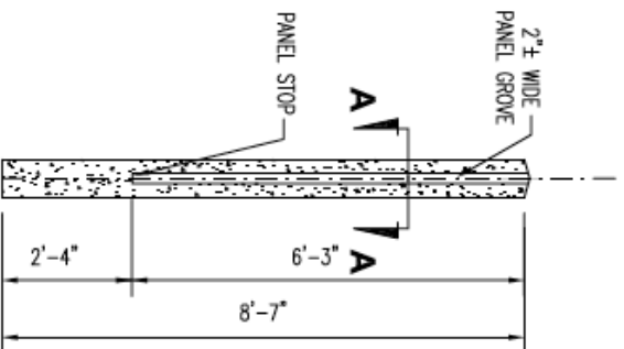
Concrete Post
